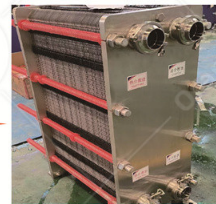
6. Plate Heat Exchanger
